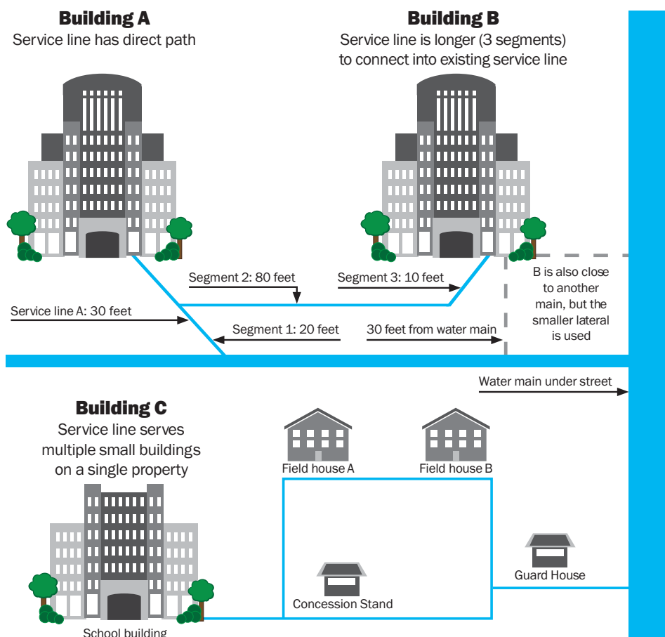
Figure 5. Examples of different building service line designs
