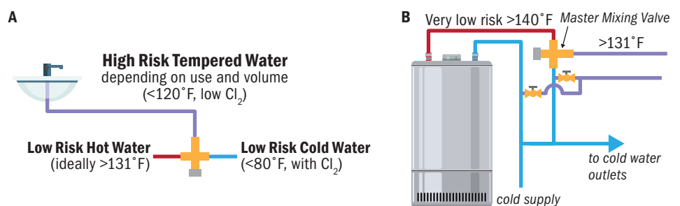
Figure 4. A) Local mixing valves supplying tempered water (<120 °F) to multiple outlets B) Centrally located master mixing valves used to temper hot water from very high temperatures in the water heater or hot water storage tank to temperatures that are safe to distribute. A mechanical master mixing valve is displayed; electronic master mixing valves are also available and more accurately control distributed hot water temperature.
